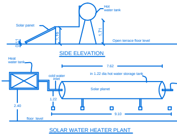
SOLAR WATER HEATER PLANT
