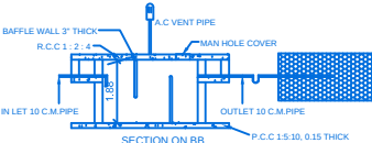
SECTION ON BB
