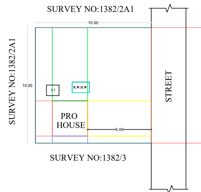
SITE PLAN
