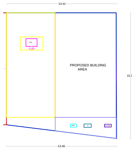
RESIDUARY PLOT SKETCH SUPER IMPOSED (SITE PLAN)
