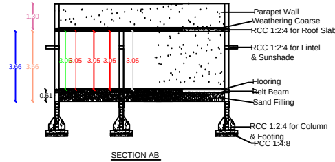
SECTION AB
