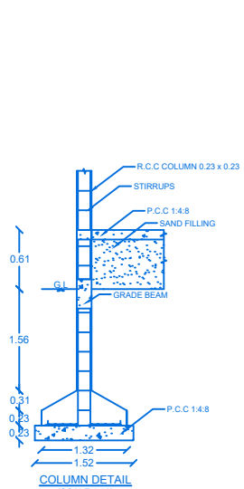
COLUMN DETAIL (SCALE 1:50)
