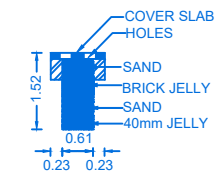
SECTION OF RAIN WATER COLLECTION TANK
