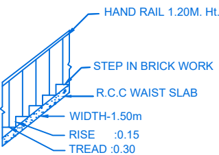
STAIR DETAIL
