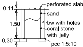
percolation pit
