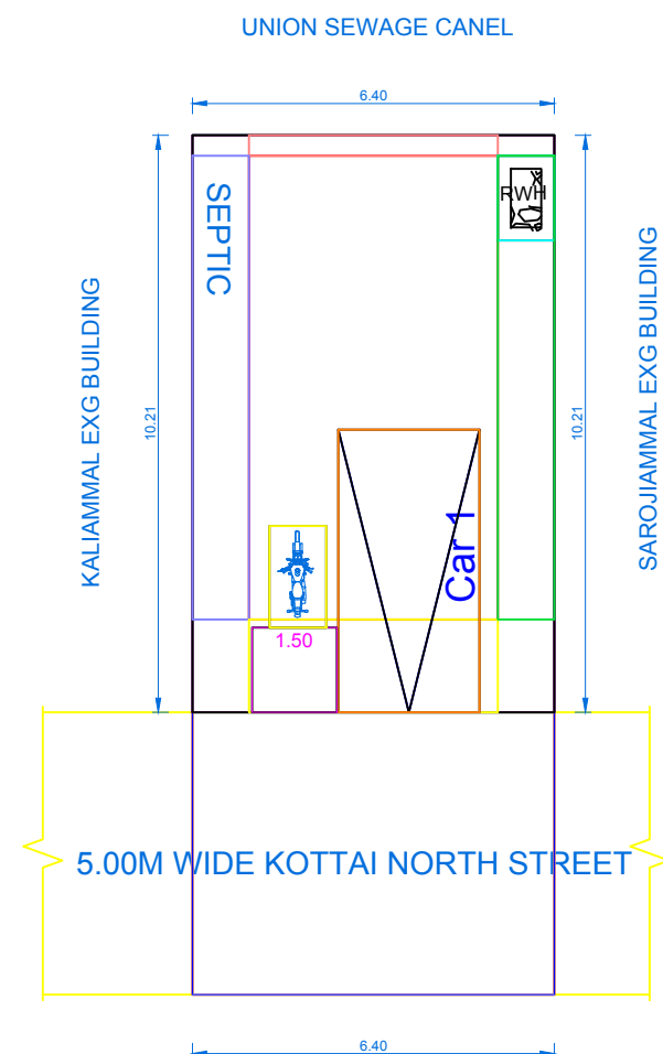
SITE PLAN
