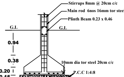
Details of coloumn footing
