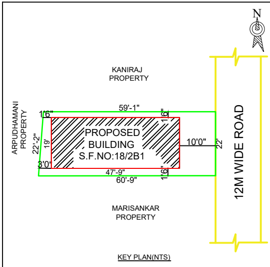
KEY PLAN(NTS)
