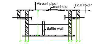
SEPTIC TANK DETAILS (NTS)
