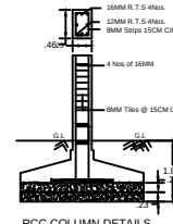
RCC COLUMN DETAILS
