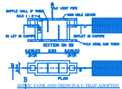
SEPTIC TANK AND TRENCH & ULTRAP ADOPTED.
