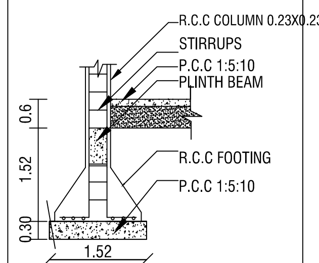
COLOUMN DETAILS
