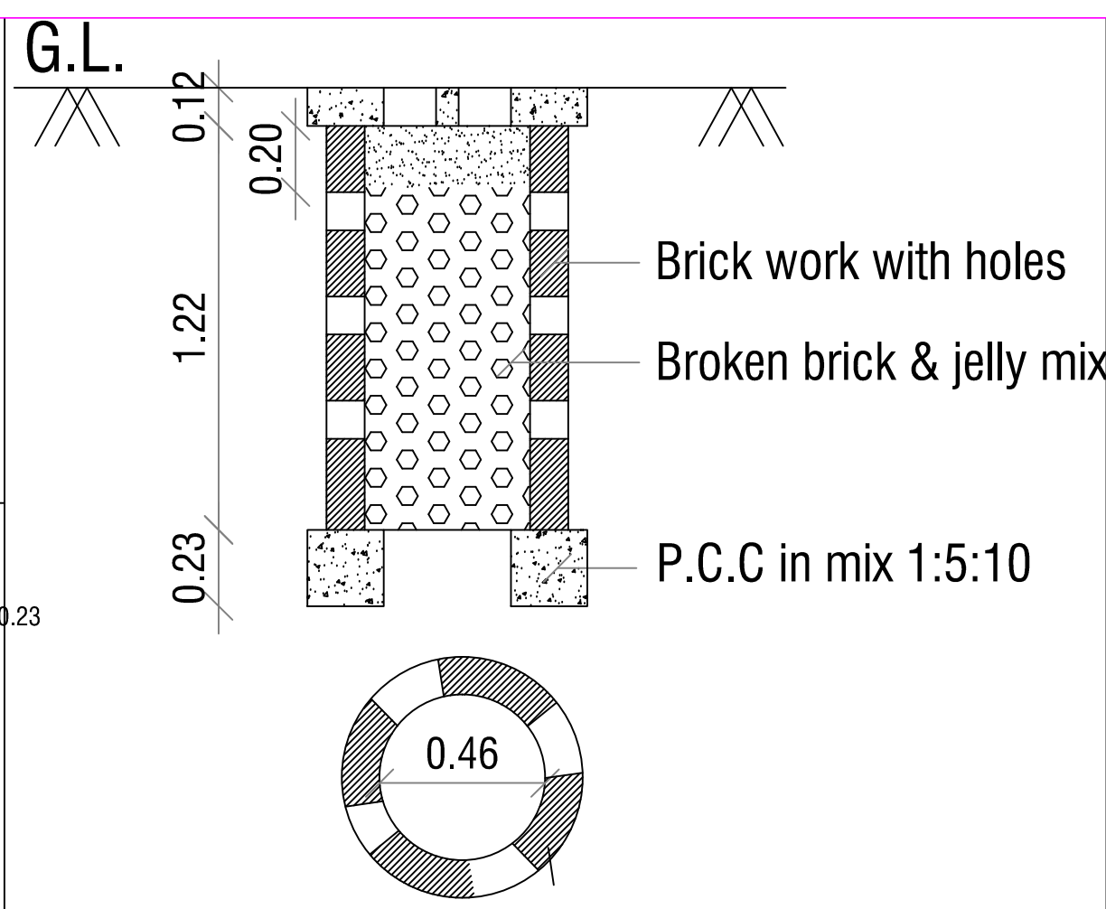
PERCOLATION PIT FOR 30 Sq. m.
