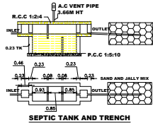
SEPTIC TANK AND TRENCH
