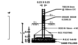
RCC COLUMN DETAILS
