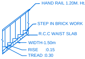
STAIR DETAIL
