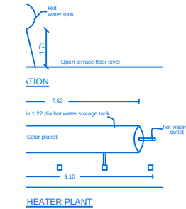
HEATER PLANT
