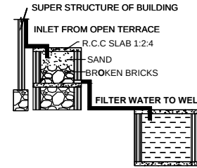
RAINWATER HARVESTING
