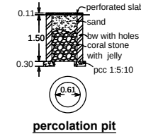
percolation pit
