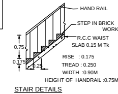
STAIR DETAILS
