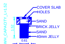
SECTION OF RAIN WATER COLLECTION TANK
