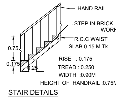
STAIR DETAILS
