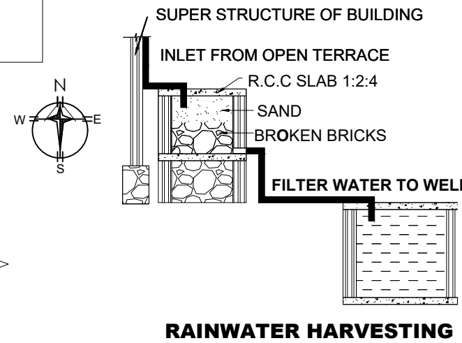
RAINWATER HARVESTING
