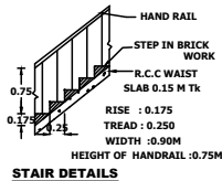
STAIR DETAILS
