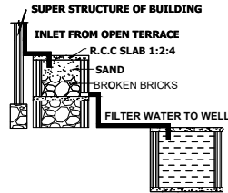
RAINWATER HARVESTING
