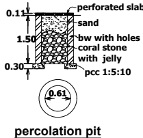
percolation pit
