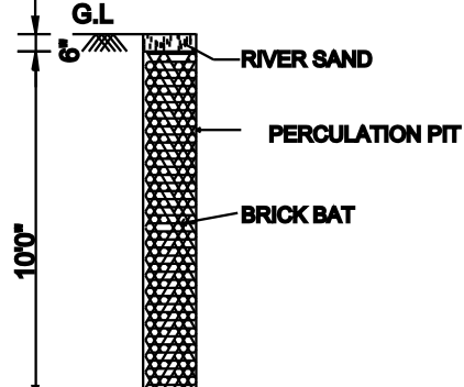
PERCOLATION PIT
