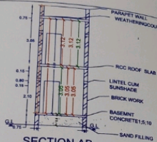
SECTION AB
