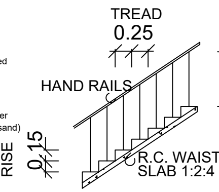
STAIRCASE DETAILS
