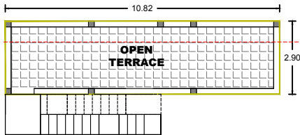
PROPOSED TERRACE PLAN
