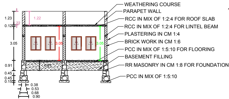
CROSSSECTION A-A'
