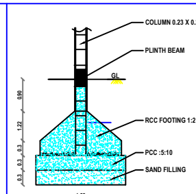
COLUMN DETAILS
