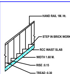
STAIR DETAIL
