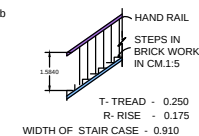
DETAILS OF STAIRCASE
