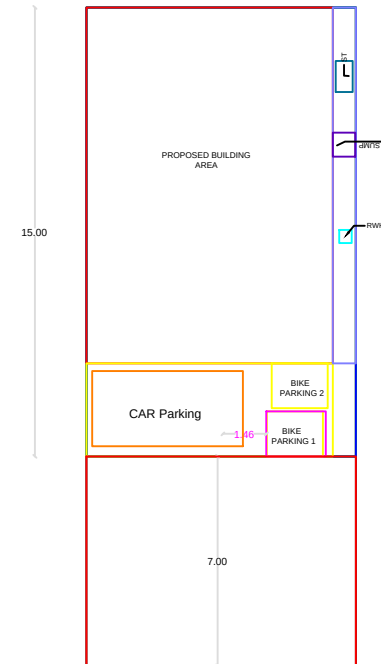
RESIDUARY PLOT SKETCH, SUPER IMPOSED SKETCH (SITE PLAN)
