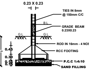
RCC COLUMN DETAILS
