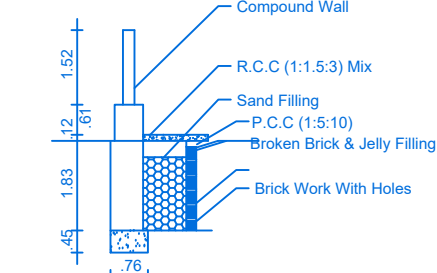
RAIN WATER HARVEST DETAILS
