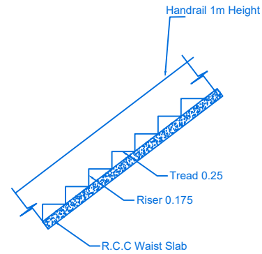
STAIR DETAILS
