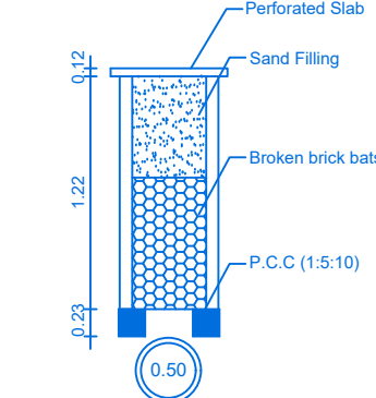
RAIN WATER COLLECTION WELL
