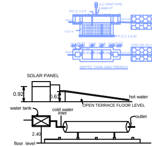
Details of solar water heating system
