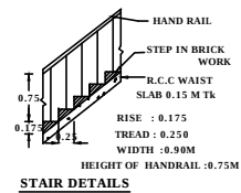
STAIR DETAILS
