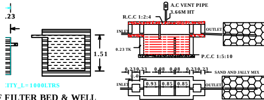
SEPTIC TANK AND TRENCH
