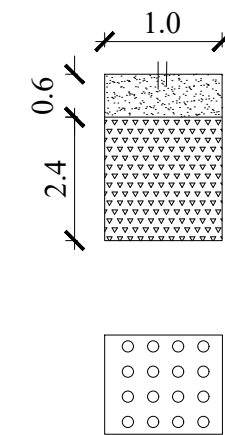
DETAIL OF RAIN WATER COLLECTING PIT- N.T.S
