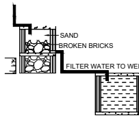
RAINWATER HARVESTING
