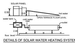
DETAILS OF SOLAR WATER HEATING SYSTEM
