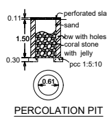
PERCOLATION PIT
