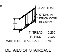
DETAILS OF STAIRCASE
