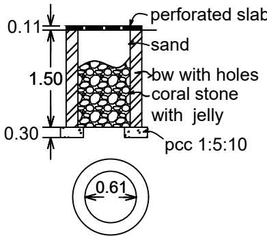
PERCOLATION PIT
