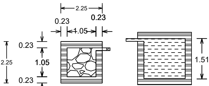
DETAILS OF FILTER BED & WELL
