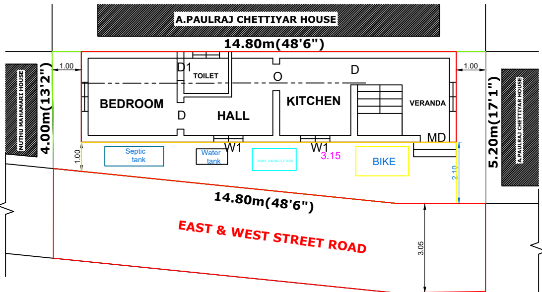
SITE PLAN
