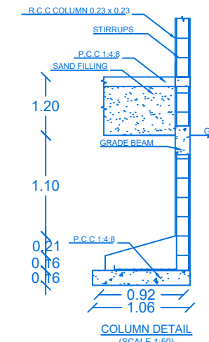
COLUMN DETAIL (SCALE 1:50)
