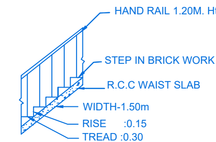
STAIR DETAIL
