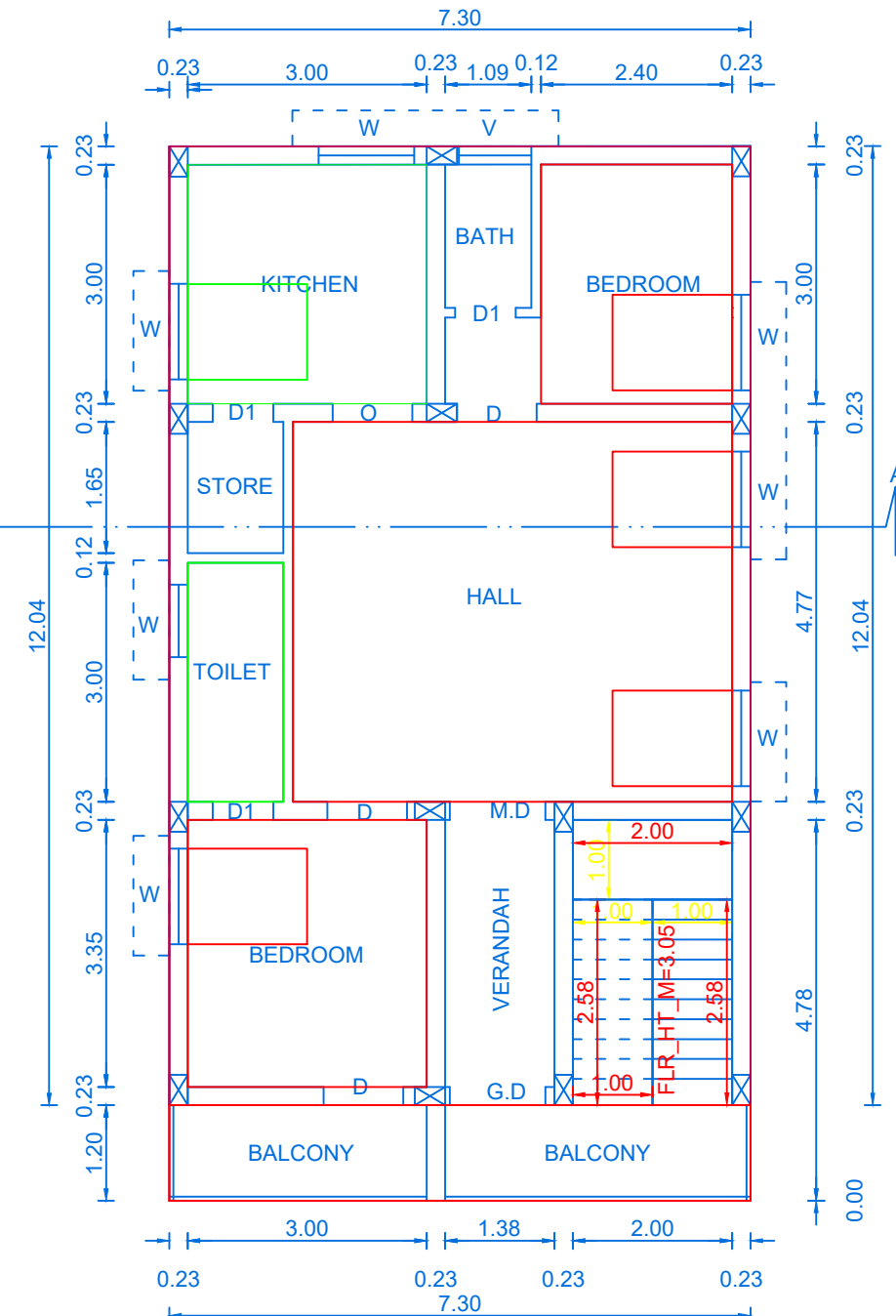
FIRST FLOOR
