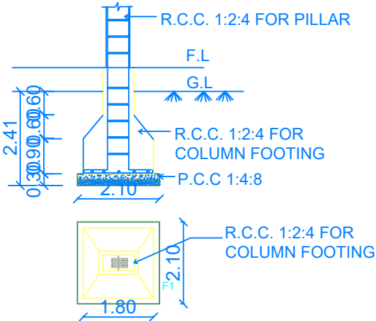
TYPICAL FOOTING
