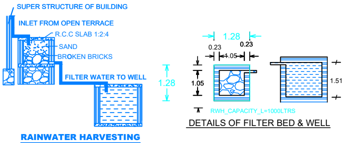
RAINWATER HARVESTING
