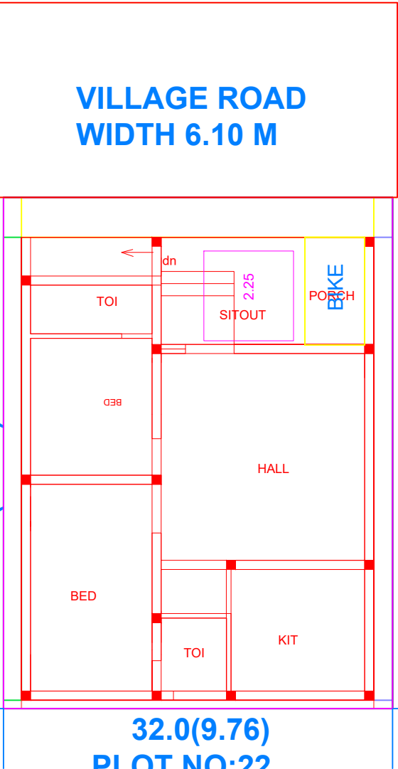
SITE PLAN
