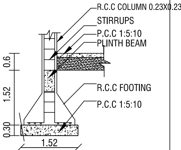
COLOUMN DETAILS
