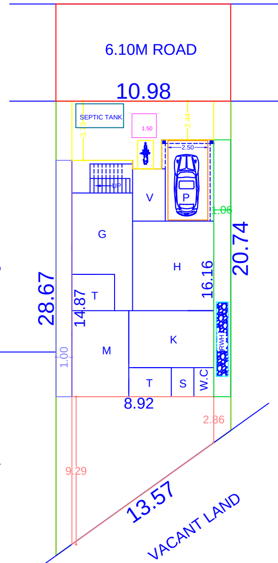
PLAN OF SEPTIC TANK & DISPERSION TRENCH
