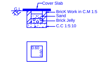
PLAN & SECTIONAL ELEVATION OF RAIN WATER HARVESTING SCALE : 1:50
