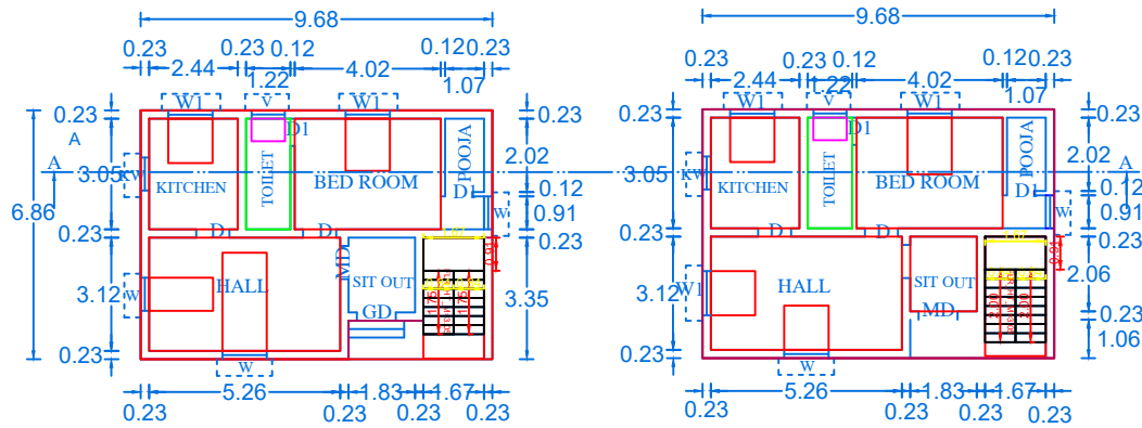
FIRST FLOOR
