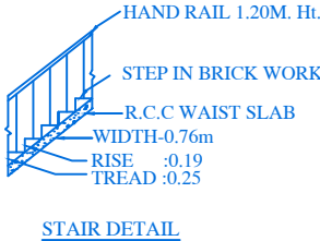
STAIR DETAIL
