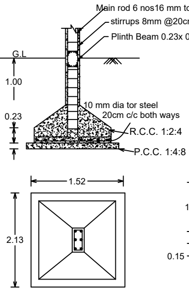
details of column footing
