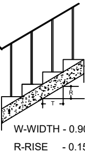
Staircase Details
