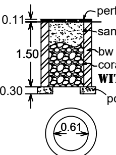
percolation pit
