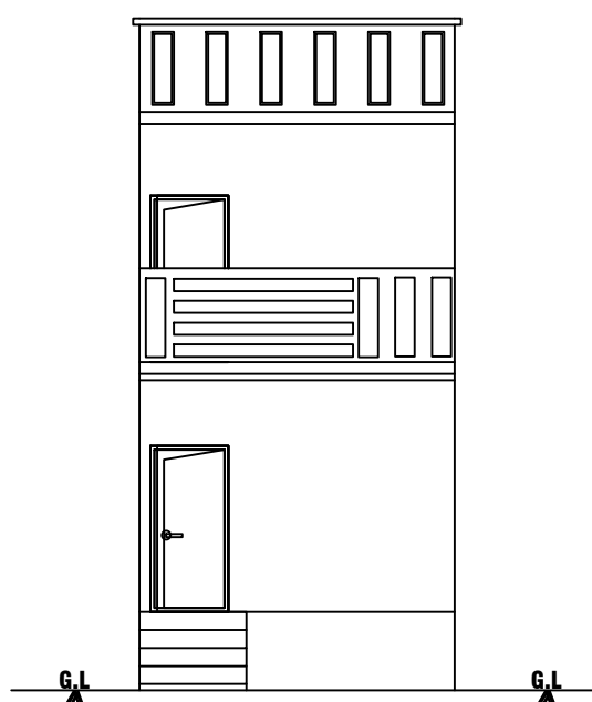
FRONT ELEVATION
