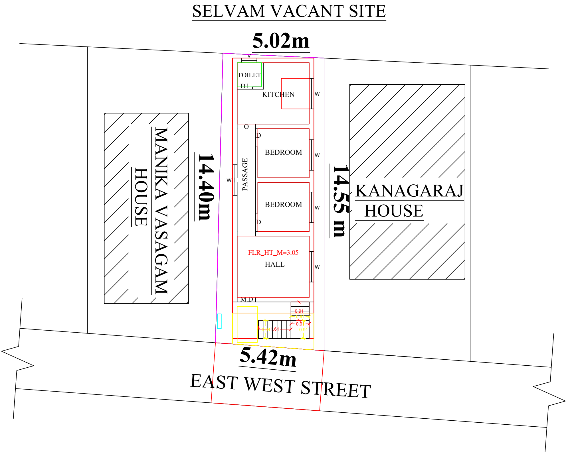
SITE PLAN(1:100)
