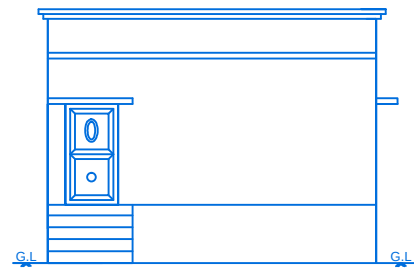
FRONT ELEVATION
