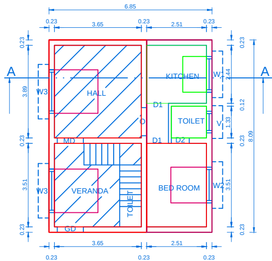
EXG & PROP.GROUND FLOOR PLAN
