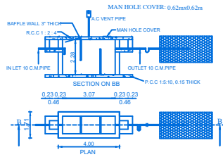
SEPTIC TANK AND TRENCH & U TRAP ADOPTED
