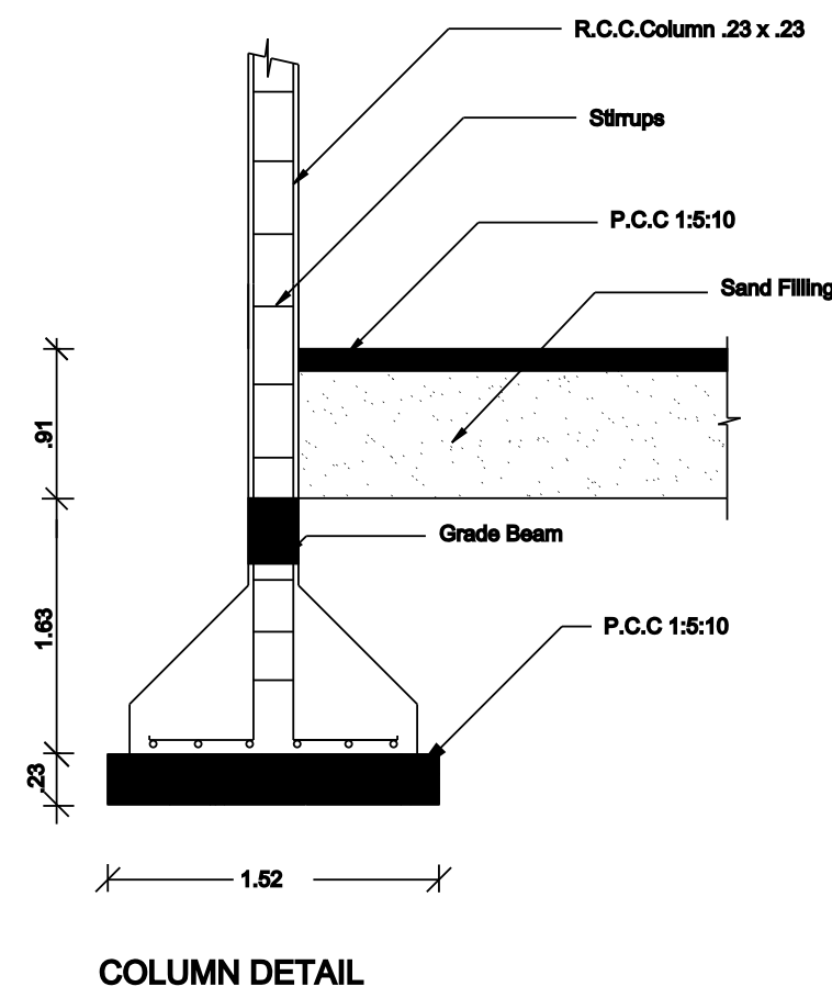
COLUMN DETAIL
