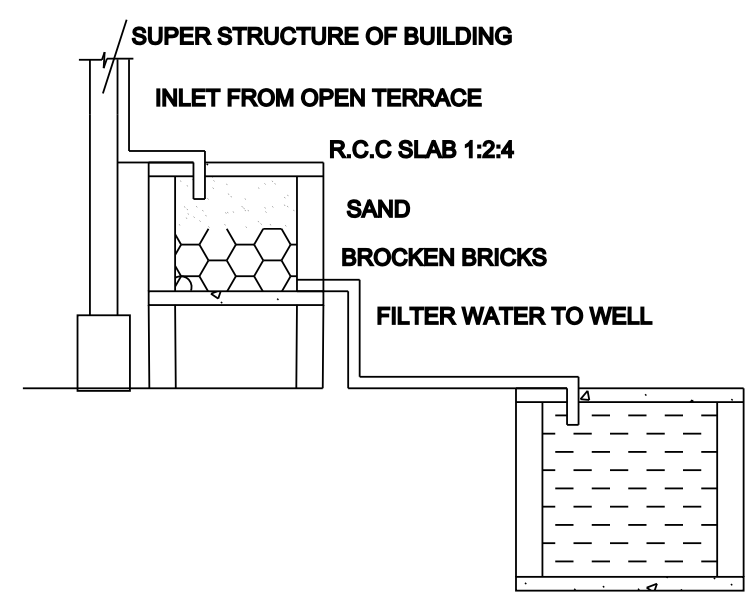
RAINWATER HARVESTING
