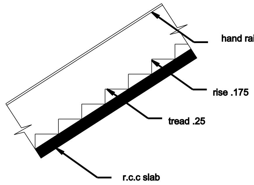
STAIR
