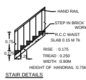
STAIR DETAILS
