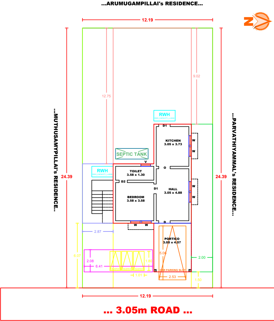
SITE PLAN FOR THE PROPOSAL
