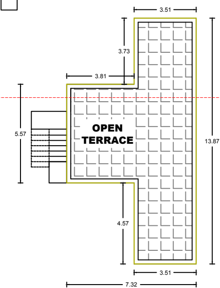
TERRACE PLAN OF THE PROPOSAL
