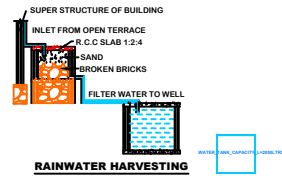
RAINWATER HARVESTING
