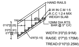
STAIRCASE DETAILS
