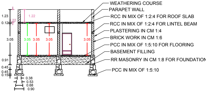
CROSSSECTION A-A'
