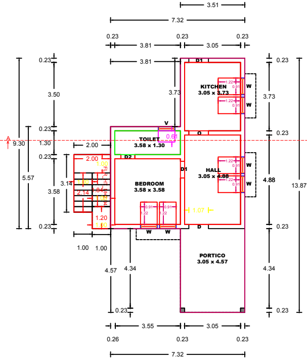
GROUND FLOOR PLAN OF THE PROPOSAL
