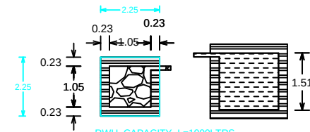
DETAILS OF FILTER BED & WELL
