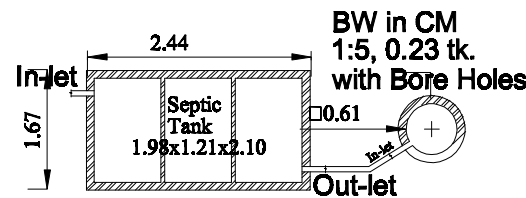
SEPTIC TANK & SOAK PIT
