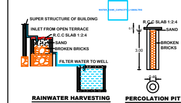
RAINWATER HARVESTING
