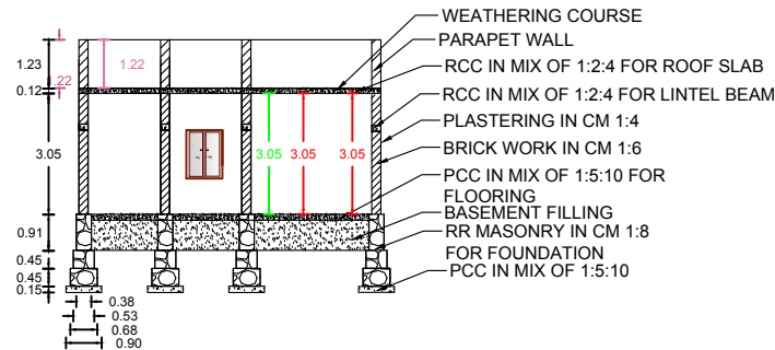
CROSSSECTION A-A'
