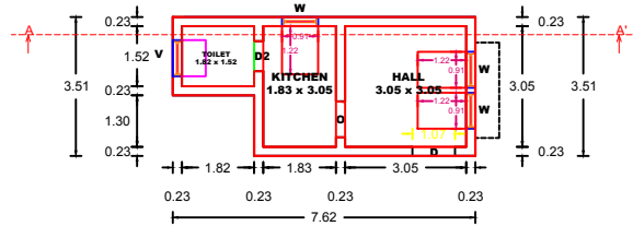
PROPOSED GROUND FLOOR PLAN
