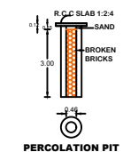
PERCOLATION PIT
