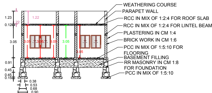
CROSSSECTION A-A'
