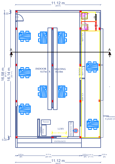
ADD.GROUND FLOOR PLAN
