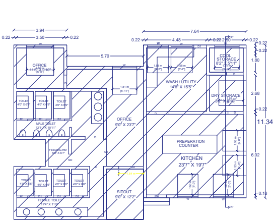
EXIST GROUND FLOOR PLAN
