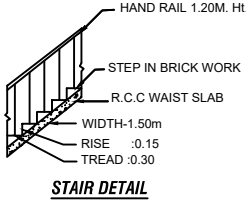
STAIR DETAIL
