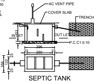
SEPTIC TANK
