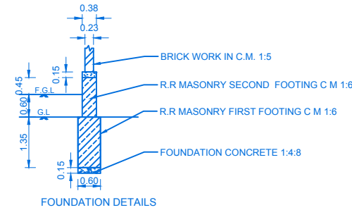
FOUNDATION DETAILS
