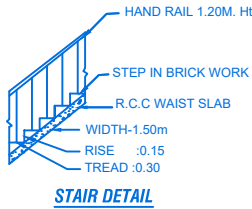
STAIR DETAIL
