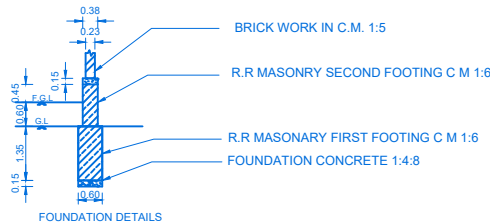
FOUNDATION DETAILS
